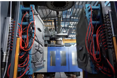
开合模 Mold Clamping Mechanism
