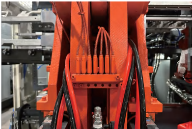
HS-自动润滑系统 HS-Automatic Lubrication System
