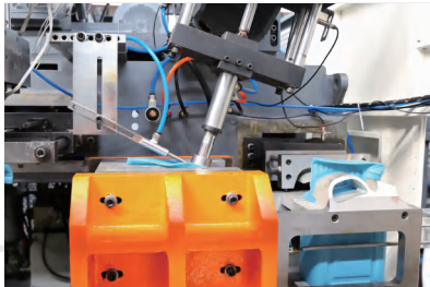
HTS-斜口瓶吹针 HTS-Beveled Blow Pin
