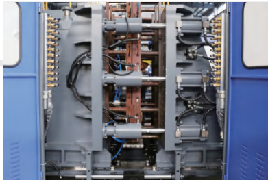
无拉杆技术 Tie-bar-less Technology
