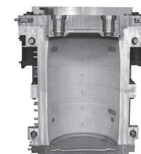
200L双口L环桶模具 200L Double L ring bucket mold
